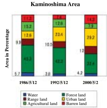
Fig. 13 Land Cover Change of Kaminoshima Area
