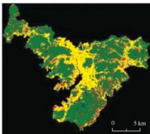
Fig. 6 Result of Land Cover Classification, 2000/5/2
