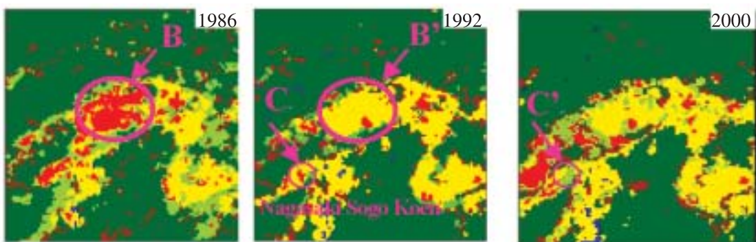
Fig. 9 Land Cover Classification Images of Koebaru in 1986, 1992 and 2000
