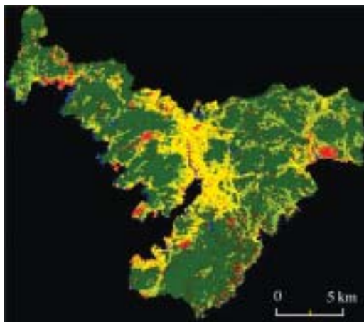
Fig. 4 Result of Land Cover Classification, 1986/5/12
