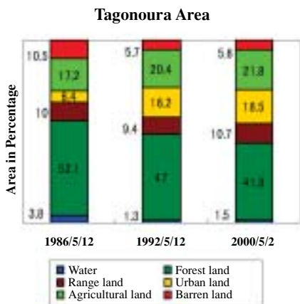
Fig. 11 Land Cover Change of Tagonoura Area
