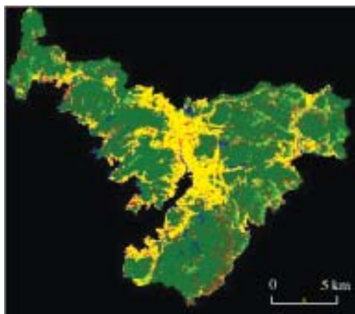
Fig. 5 Result of Land Cover Classification, 1992/5/12
